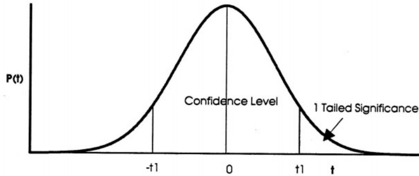
Figure H.1: The t distribution
