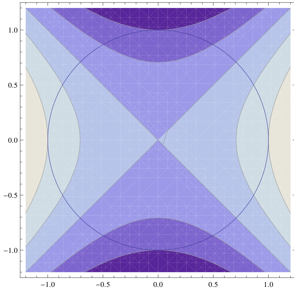
Figure 1: Contour plot of f(x, y) = x^2 - y^2 with the curve x^2 + y^2 = 1 .
